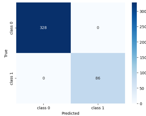
Figure 3. Classification report data publik metode original
