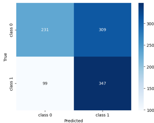
Figure 6. Classification report data privat metode augmentasi
