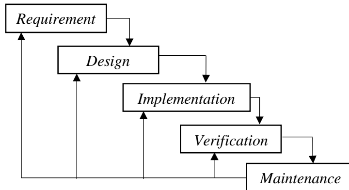
Gambar 2.1 - Metode Waterfall
