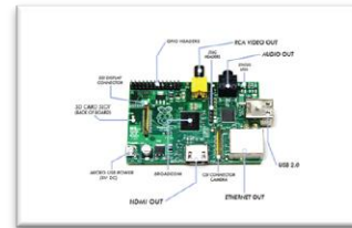
Gambar 2.1 Raspberry Pi
