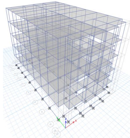
Gambar 2 . Program Etabs
